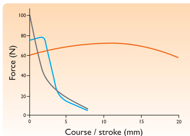
— Linear solenoid — Proportional solenoid — Voice coil
