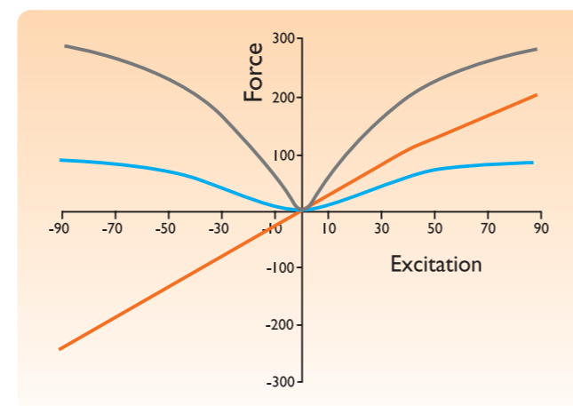
— Linear solenoid — Proportional solenoid — Voice coil
